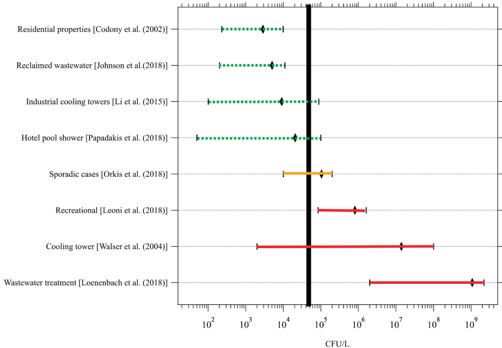
FIGURE 3-9 Concentrations of culturable Legionella during outbreaks and routine monitoring from various environments (ranges shown as bars, averages shown as diamonds). Red solid lines are outbreaks. Green dashed lines are routine sampling. The orange solid line is from sporadic cases. The solid black line is the 5 \times 10^4 CFU/L action level identified by the Committee as a break between sporadic cases and outbreaks.
