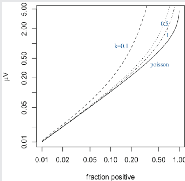
FIGURE 3-12-1 Estimation of mean number given fraction of positive samples for Poisson vs. negative binomial distributions.
