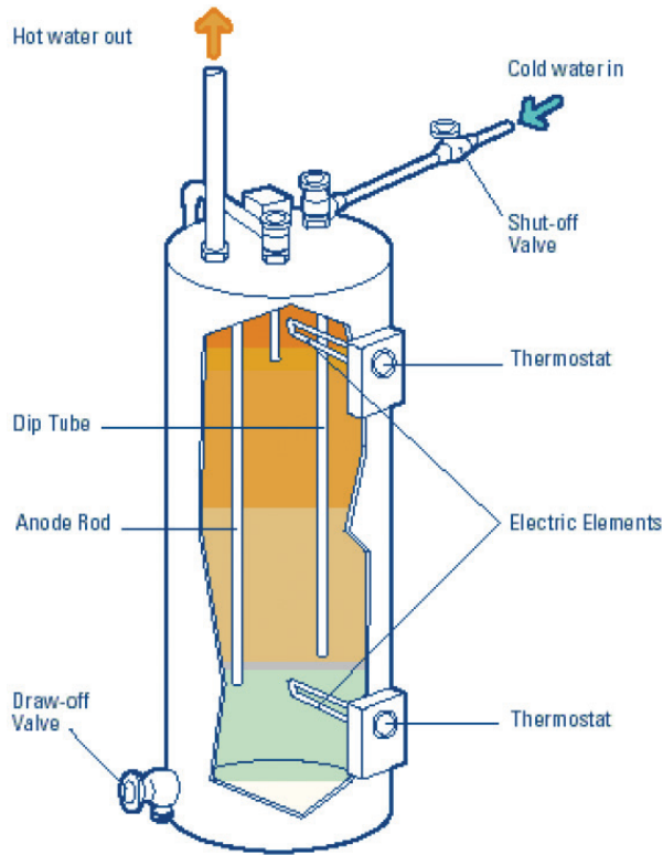
FIGURE 1-9 Schematic of an electric hot-water heater and photo of a gas hot-water heater.
