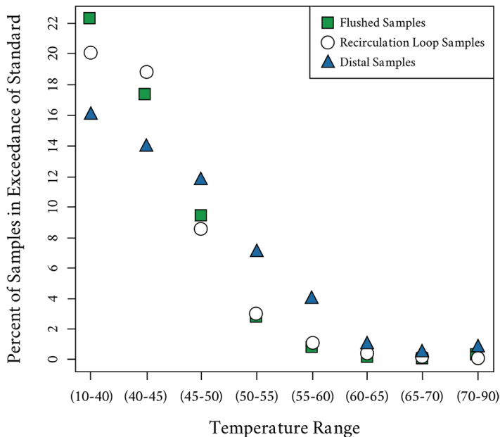
FIGURE 4-2 Relationship between temperature (x-axis) and the percentage of samples exceeding the German standard of 100 CFU/100mL (y-axis) for Legionella spp. from public buildings in Germany over a seven-year period. The squares are for flushed samples, the triangles are distal samples, and the circles are samples from the recirculation loop. SOURCE: Kistemann and Wasser (2018).
