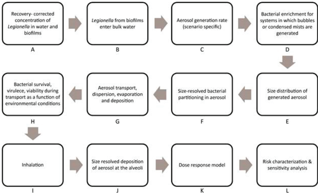
FIGURE 3-10 Framework for Legionella QMRA.
