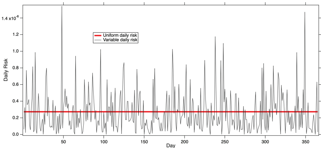
FIGURE 3-12 Sketch of uniform daily risk vs. variable daily risk.
