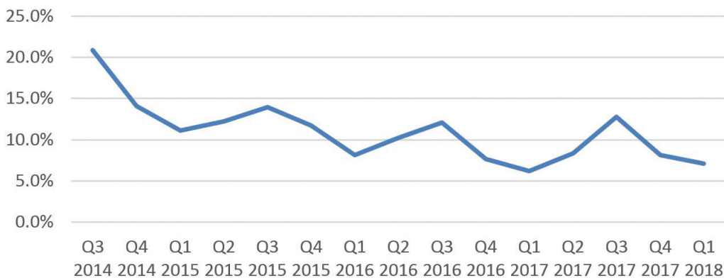
FIGURE 5-2 Percentage of Quebec cooling towers with L. pneumophila serogroups 1-14 concentrations exceeding 10^4 CFU/L over time.
