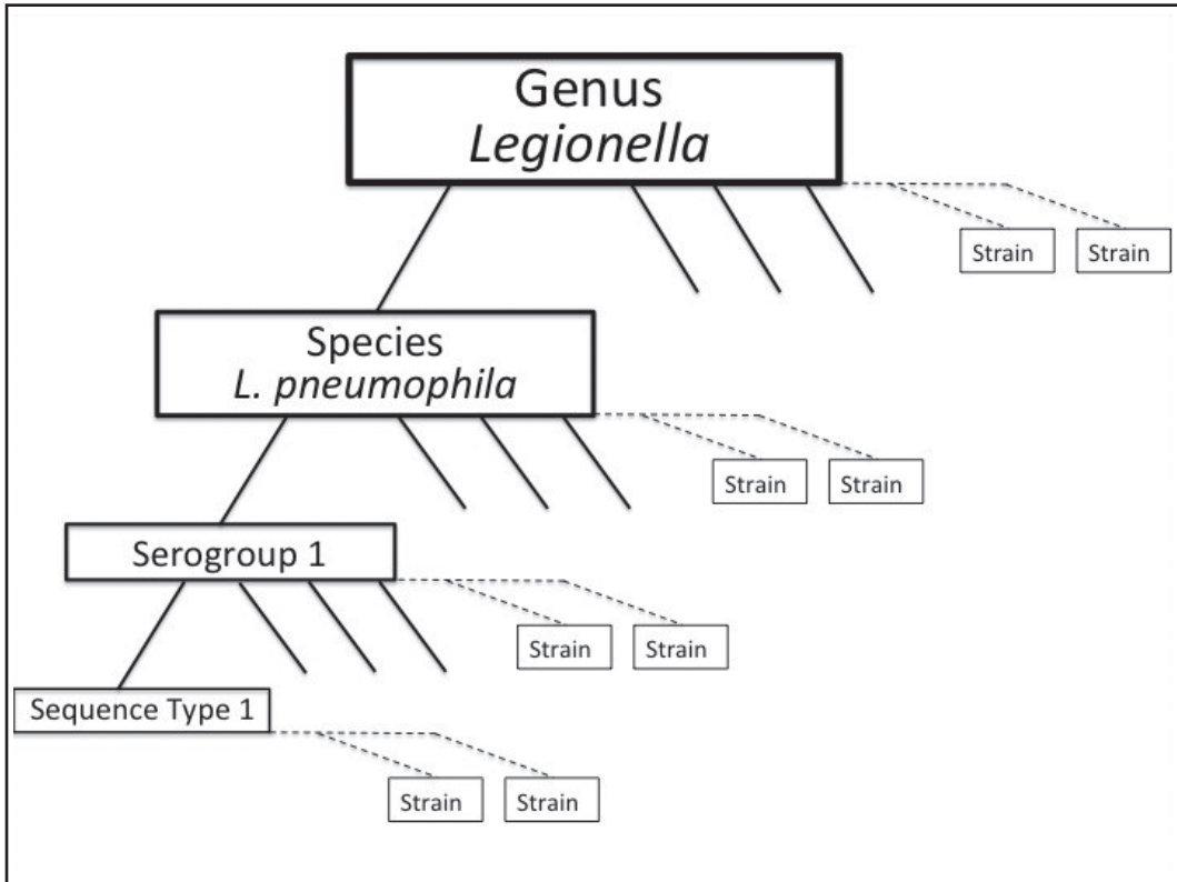
FIGURE 2-4 Nomenclature of Legionella . Genus and species are taxonomic categories that denote the degree of similarity among organisms. Serogroup refers to a distinct antigenic profile of the outer membrane lipopolysaccharide. Sequence type is defined by the DNA sequence of seven genomic loci designated by the field. Strain (dashed lines) is a more general term used to distinguish bacterial isolates without reference to their genetic or antigenic identity; for example, L. pneumophila cultures isolated independently are initially given different strain names until additional information on species, serogroup, or sequence type is obtained.
