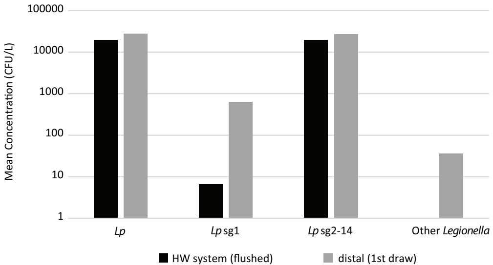
FIGURE 4-3 Concentrations of various Legionella species and strains in Italian hospital water systems. First-draw samples reflect conditions at the distal ends, while flushed samples represent conditions in the main hot-water system.
