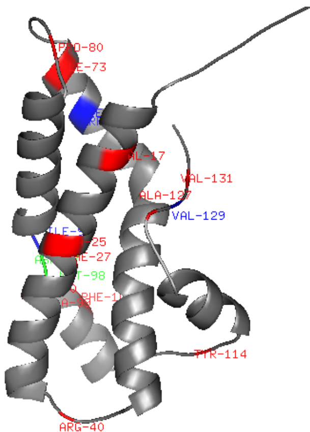
Figure 3 Lysin crystal structure from the red abalone Haliotis rufescens ([24], PDB ID 1ILS). Sites in color are in the ( \omega \leq 1 , \gamma \geq 1 ) category. Sites that are blue (68,69,96,129) are from the volume and charge partitions. Sites that are red (17,5,27,30,40,73,80,99,101,114,127,131) are from the volume partition only. Finally, sites that are green (97–98) are from the charge partition only.
